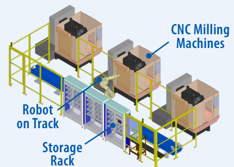
Milling Robot-on-Track Cell (MRTC)
