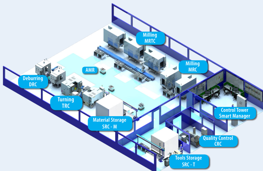
Smart Factory for Precision Manufacturing
