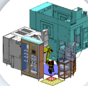
Turning Milling Robotic Cell (TMRC)
